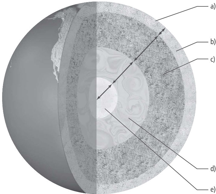
Layers of the Earth
